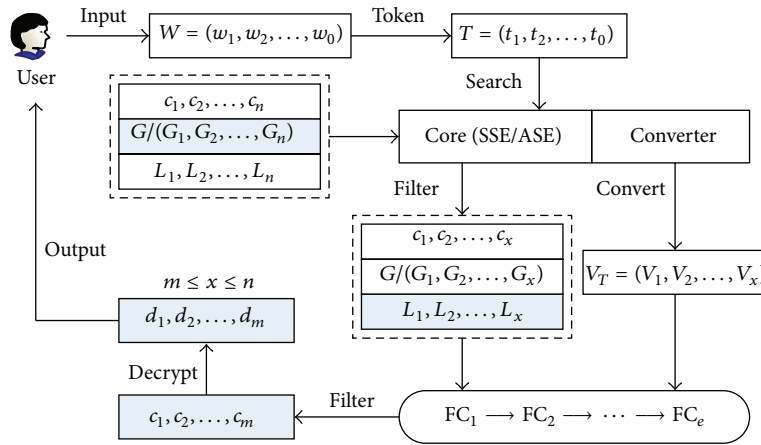
FIGURE 2: Search process of layered searchable encryption scheme.
