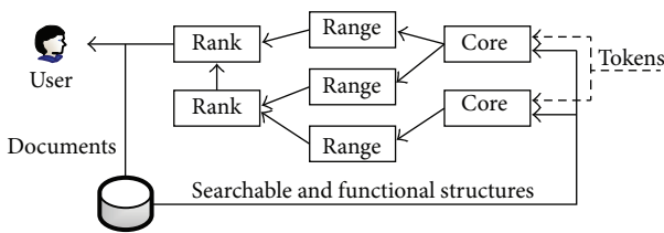
FIGURE 5: Deploying functional components to multiple servers.
